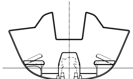
SECTION AT STN. 6
