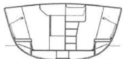
SECTION AT STN 5.33 (Looking AB)
