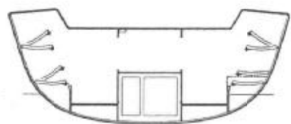
SECTION AT STN 7
