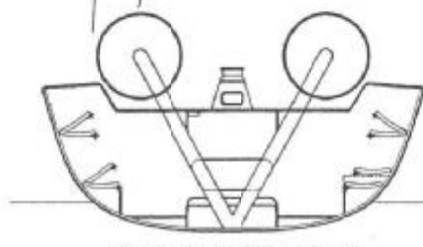
SECTION AT STEERING PEDESTALS
