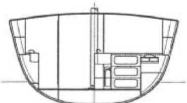
SECTION AT STN 4.87 (Looking Port)
